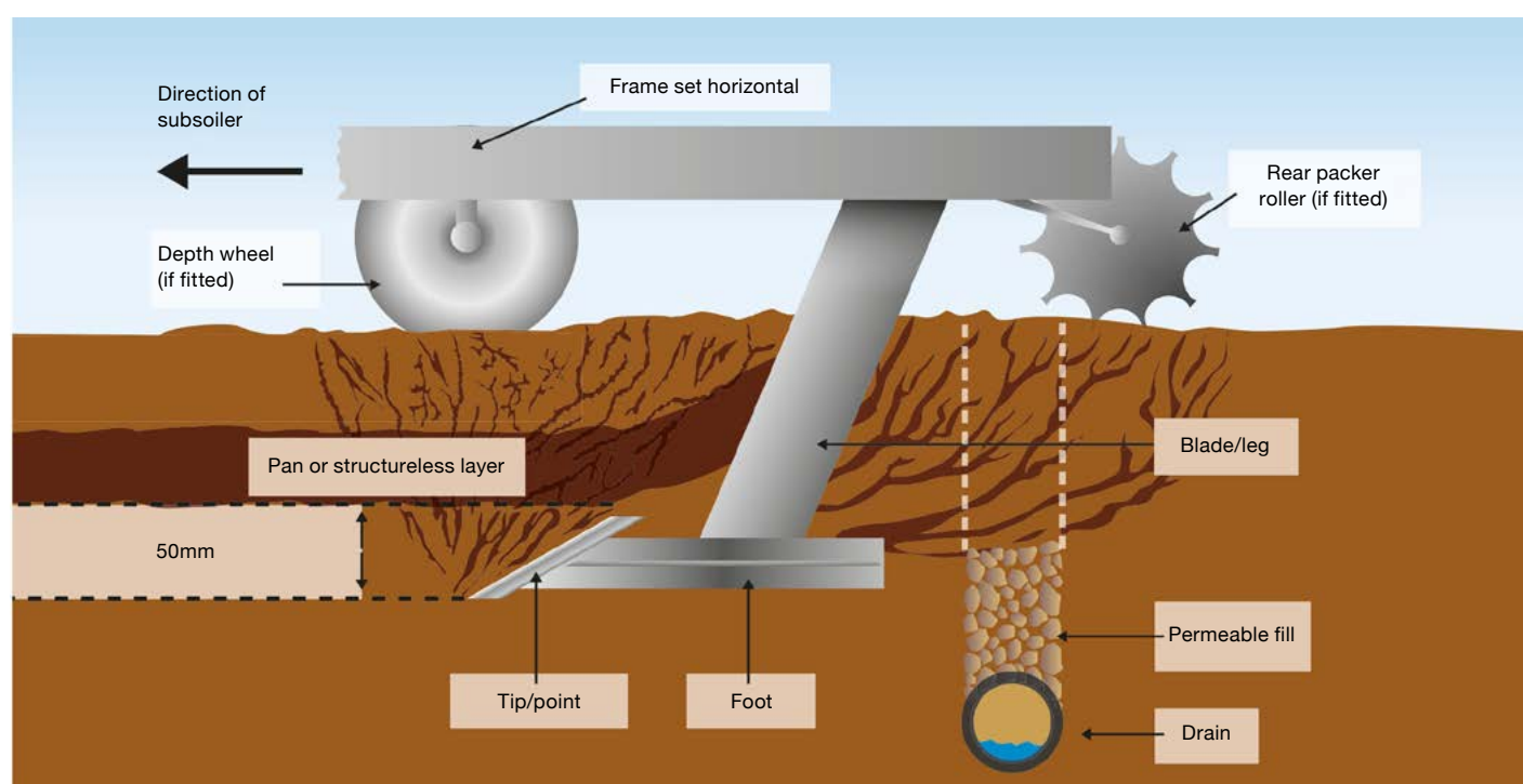
Figure 13. Subsoiler operation
